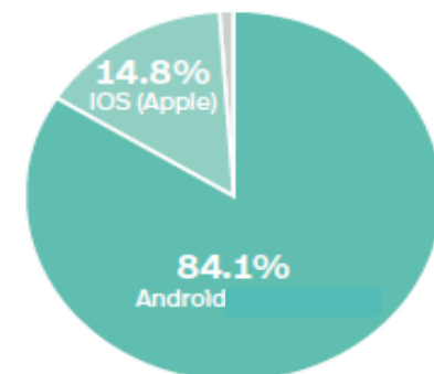
Smartphone OS 2)
